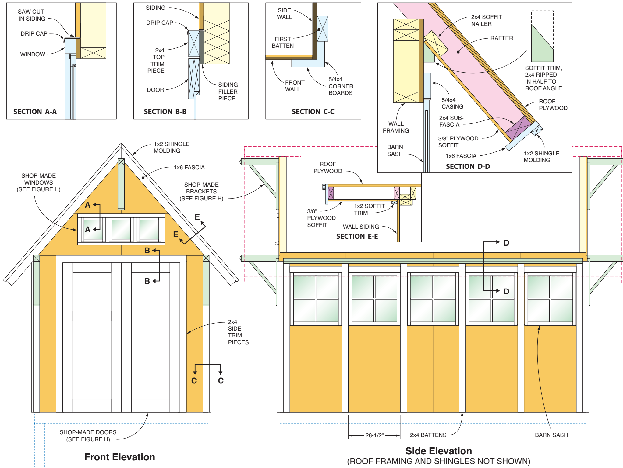
Figure G. Shed details
